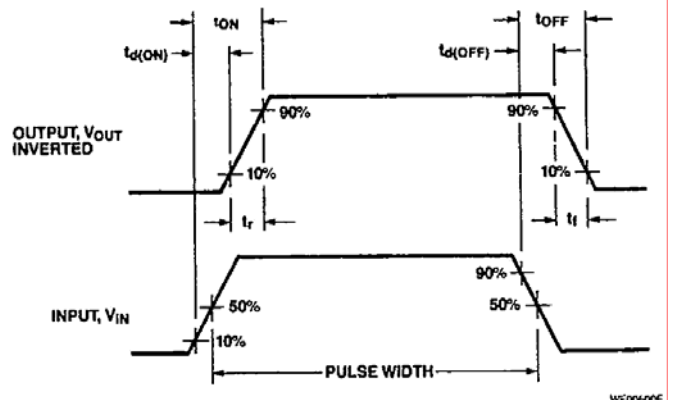
Figure 10 Switching Waveforms
