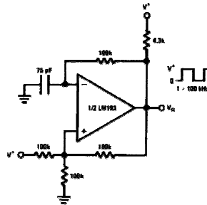
Squarewave Oscillator
