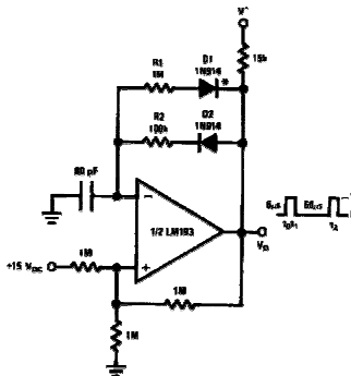
Pulse Generator
