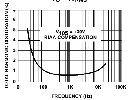
Distortion vs Frequency V_O = 1\text{V}_{\text{RMS}}
